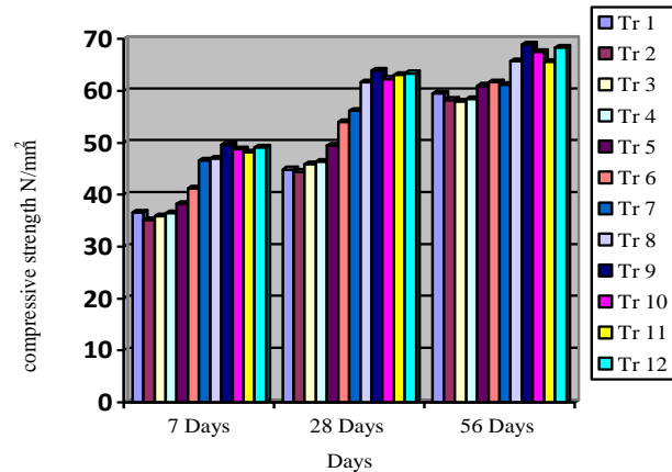
Figure 5: Cube Compressive Strength \text{N/mm}^2 (SCC)
