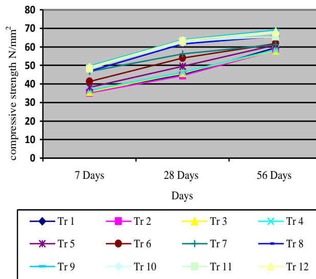
Figure 6: Cube Compressive Strength \text{N/mm}^2 (SCC)
